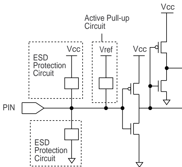
Typ. V_{ref} = 3.2V
