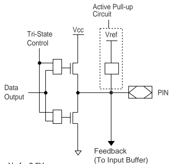
Typ. V_{ref} = 3.2V
